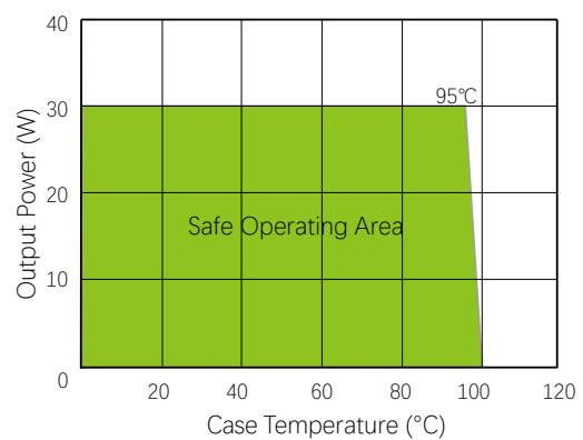
THERMAL DERATING
