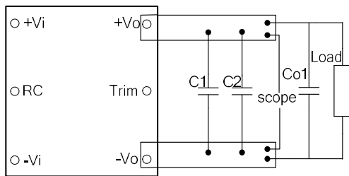
Figure 4: Output Ripple & Noise
