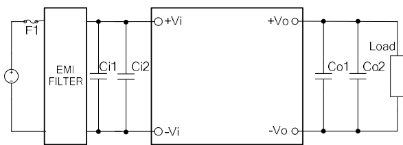
Figure 1: Typical Application Connection Single Output
