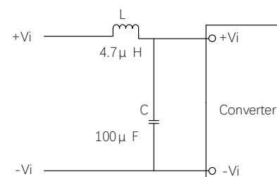
Figure 4: Reflected Ripple Current
